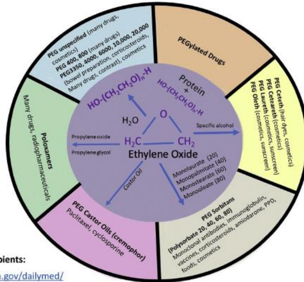
FIGURE 2. Excipients whose chemical derivation uses ethylene oxides, some of which have demonstrated clinical cross reactivity in PEG allergic patients. PEG, Polyethylene glycol; PPD, purified protein derivative.
